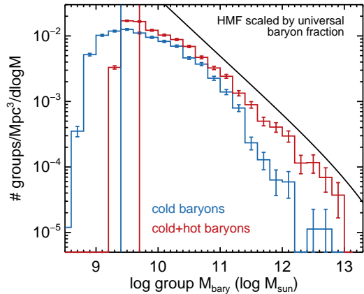
Figure 14. ECO group CBMF (blue) and BMF including hot X-ray gas (red), where we used the hot gas prescription based on dark matter halo mass from Giodini et al. (2009), scaled for our halo mass definition. The completeness limits are shown as vertical lines corresponding to the colors of the histograms. The BMF completeness limit is determined by finding the maximum hot gas correction to group M_{\text{bary}}^{\text{cold}} at 10^{9.4} M_{\odot} , which we find to be \sim 0.3 dex. Including the hot gas causes the group BMF to run parallel to the dark matter HMF. In this analysis for simplicity we do not use full group mass likelihood distributions but instead median values. Error bars represent the Poisson statistics.
