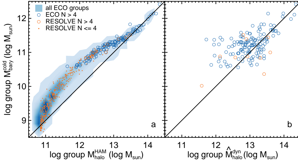
Figure 1. Group M_{\text{bary}}^{\text{cold}} (including satellite completeness corrections, see §2.4) vs. M_{\text{halo}} measured by (a) HAM and (b) dynamical estimates. ECO is shown in blue and RESOLVE is shown in orange. The black line shows a one-to-one relationship shifted down by 2 dex. Groups with N > 4 are shown as open circles. M_{\text{halo}}^{\text{HAM}} is closely correlated to the group M_{\text{bary}}^{\text{cold}} since we have used group r -band luminosity (group L_r ) to perform the abundance matching and L_r correlates closely with cold baryonic mass (K13). Dynamical estimates are shown only for groups with N > 4 members and show larger scatter with baryonic content at lower halo masses due to having fewer members for the dynamical mass calculation.
