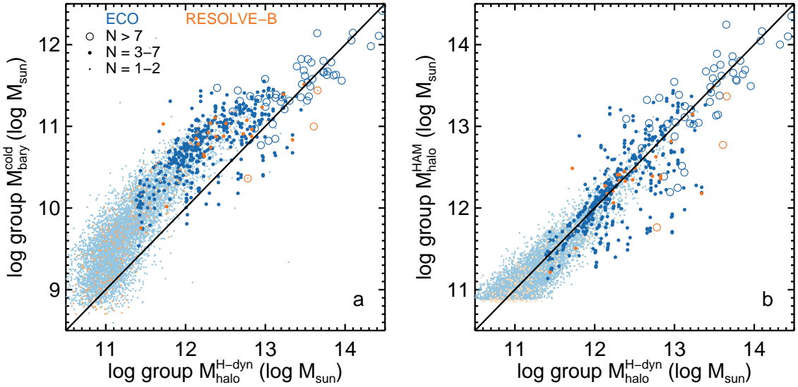
Figure 4. (a) Group M_{bary}^{cold} (including satellite completeness corrections) and (b) M_{halo}^{HAM} vs. M_{halo}^{H-dyn} using direct and stacking measurements at large N and stacking measurements and HAM at low- N . ECO is shown in blue and RESOLVE is shown in orange. The black line shows a one-to-one relationship shifted down by 2 dex in panel (a) and a one-to-one relationship in panel (b). Groups with N > 7 are shown as open circles, while groups with 3 \leq N \leq 7 are shown as medium sized dots and groups with N = 1 and 2 are shown as small dots. Groups are assigned mass according to group \bar{N} as described in §2.3.5.
