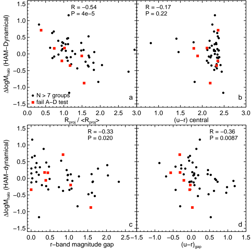
Figure 2. Residual correlations between \Delta\log M_{halo} and (a) R_{proj}/\langle R_{proj} \rangle the projected radius normalized to the median projected radius at a given group L_r , (b) u-r color of the central, (c) r -band magnitude gap, and (d) u-r color gap. Only groups with N > 7 members are shown, and \Delta\log M_{halo} is computed as the difference between the log of M_{halo}^{HAM} and the log of \hat{M}_{halo}^{dyn} (scaled by A = 9.9 ). Groups that fail the A-D test (i.e., that are not virialized) are shown in red. The Spearman rank correlation coefficient and probability of no correlation are reported as R and P respectively. R_{proj}/\langle R_{proj} \rangle yields the most significant correlation with \Delta\log M_{halo} with the highest coefficient of correlation and the least scatter. The color of the central does not show a significant correlation with \Delta\log M_{halo} . The r -band magnitude gap and u-r color gap do show significant correlations with \Delta\log M_{halo} , although with smaller coefficients of correlation and greater scatter than for R_{proj}/\langle R_{proj} \rangle .
