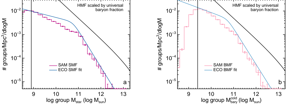
Figure 6. Group (a) SMF and (b) CBMF for the FOF groups in the GALFORM semi-analytic model. (Results are not shown for the mock catalog true groups but are similar.) Since the simulation’s stellar and baryonic mass are exact quantities, we plot the mass functions with Poisson error bars only. The theoretical dark matter HMF scaled by the universal baryon fraction is shown in black and the ECO group SMF and CBMF are also shown plotted in their respective panels. The SAM and ECO group MFs exhibit similar overall behavior, with a break in power-law slope near \sim 10^{11} M_{\odot} . The SAM, however, shows a dip in numbers relative to ECO at this mass scale and a more steeply rising slope at the lowest masses. The solid vertical lines show the stellar and cold baryonic completion limits of the ECO survey.
