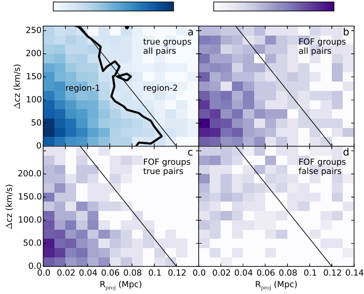
Figure 16. Mock catalog pair statistics, shown as 2-D histograms of the distribution of pairs ( N = 2 groups) over \Delta cz vs. R_{proj} space for (a) all true pairs, (b) all FOF pairs, (c) true FOF pairs, and (d) false FOF pairs. (Split-off FOF pairs are not shown, but are distributed roughly equally over this space.) The 2-D histograms for panels (b)–(d) are normalized to all FOF pairs, with the color bar shown above panel (b). In panel (a) we show the contour containing 95% of the true-mock pairs (thick black line) as well as the line we choose to define region-1 and region-2 (thin black line). Only 5% of true FOF pairs live in region-2, while nearly 50% of false FOF pairs live in region-2. We therefore break up all pairs in region-2, improving the percentage of true pairs among FOF pairs from 62% to 73%.
