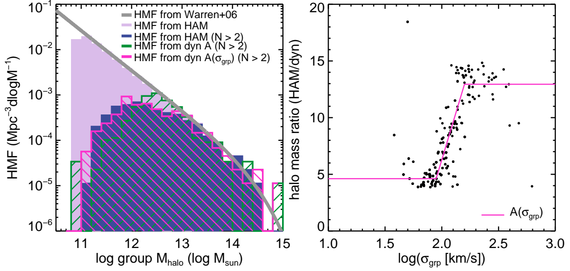
Figure 3. Method to determine the scale factor A(\sigma_{grp}) for the dynamical mass estimates (using both the direct and stacking estimates). (a) The ECO HMF for M_{halo}^{HAM} (light purple filled histogram) by construction matches the Warren et al. (2006) HMF (grey thick line). The ECO HMF for M_{halo}^{HAM} for N > 2 groups only (dark purple filled histogram) is shown for comparison to the HMF of dynamical masses. The HMF of M_{halo}^{dyn} (scaled by a constant factor of A , green crosshatched histogram) overproduces intermediate-mass groups of mass \sim 10^{12.5} M_{\odot} . The HMF of M_{halo}^{H-dyn} scaled by A(\sigma_{grp}) (pink cross-hatched histogram) is calibrated to reproduce the cumulative HMF for N > 2 groups. (b) To determine the scale factor A(\sigma_{grp}) , we find the HAM and dynamical halo masses at each group's cumulative number density and plot their ratio as a function of \log(\sigma_{grp}) . Since we do not want to account for groups of N = 1 and 2, we use the cumulative HMF from the HAM estimates and join it to the cumulative HMF from theory at high masses (where ECO has less data). To fit the data, we take the median of the halo mass ratio at high and low sigma (where the relationship is relatively flat) and fit a line between \log(\sigma_{grp}) = 1.9-2.2 (pink). This calibration is applied to the dynamical mass estimates.
