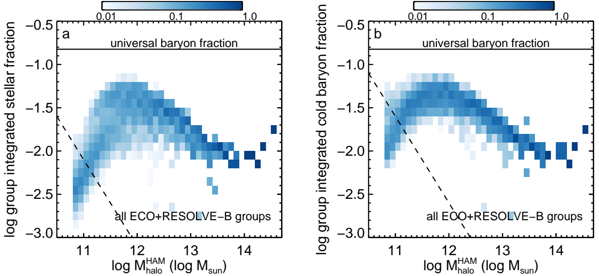
Figure 7. Conditional density plot of group-integrated (a) stellar and (b) cold baryon fraction as a function of M_{halo}^{HAM} based on group L_r for all ECO and RESOLVE-B groups. The number densities are weighted by the central completeness corrections described in §2.4. The universal baryon fraction (0.15) is shown as a line at the top and the group M_{star} and M_{bary}^{cold} completeness limits are shown by the dashed black lines. The group-integrated stellar mass fraction falls sharply above and below group halo mass \sim 10^{11.8} M_{\odot} . The group-integrated cold baryon fraction reaches a maximum over the nascent group regime ( 10^{11.4-12} M_{\odot} ) with little scatter. At high group halo mass, the stellar and cold baryon fractions are similar.
