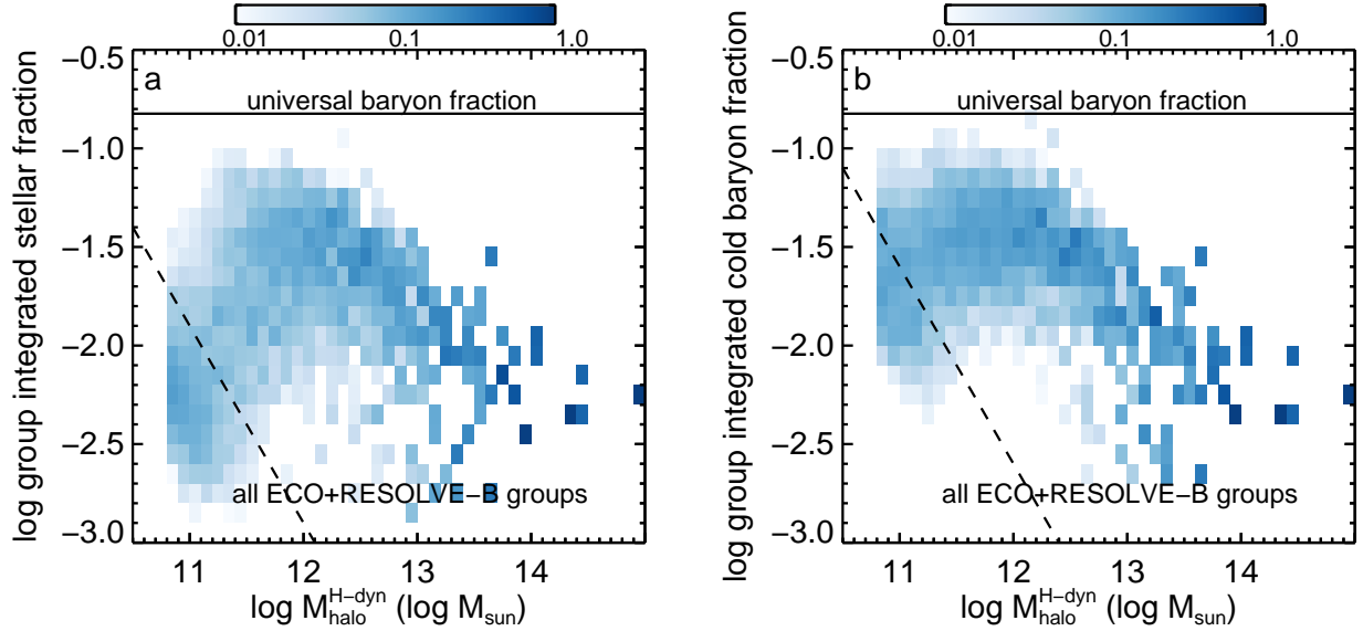
Figure 9. Conditional density plot of group-integrated (a) stellar and (b) cold baryon fraction as a function of M_{halo}^{H-dyn} determined by the combination of N \geq 3 dynamical and low-N HAM estimates for both ECO and RESOLVE-B groups combined. The universal baryon fraction is shown as a line at the top and the group cold baryonic mass completeness limit is shown by the dashed black line. Using dynamical mass results in a wider range of group stellar and cold baryon fractions, particularly over the nascent group halo mass range (and below, but here the scatter is introduced see §2.3.5). The peak baryonic collapse efficiency occurs near \sim 10^{12} M_{\odot} .
