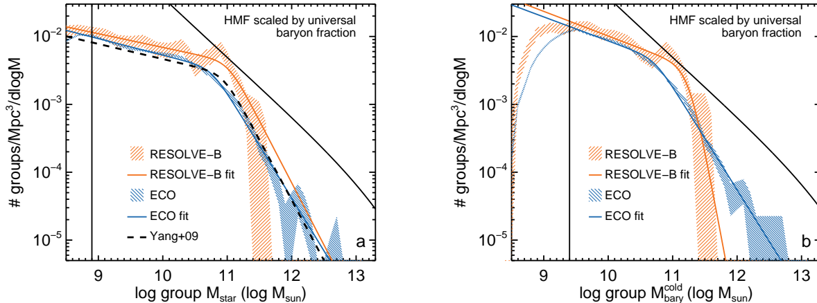
Figure 5. Group (a) SMF and (b) CBMF for ECO (blue) and RESOLVE-B (orange) determined using the cross-bin sampling method of E16. The cross-hatched regions show the 16th-84th percentile uncertainty bands and the black vertical lines designate the group M_{star} and M_{bary}^{cold} completeness limits. The theoretical dark matter HMF of Warren et al. (2006) scaled by a universal baryon fraction of 0.15 (Planck Collaboration et al. 2014) is shown in black. In both panels the group MFs fall short of the theoretical HMF at both high and low masses. The black dashed line in panel (a) shows the double power law fit to the group SMF given in Yang et al. (2009). The dark blue and orange lines in both panels show our fits using the same model for the ECO and RESOLVE group MFs. The group CBMF shows similar behavior to the group SMF at high masses and a steeper low-mass slope, as also seen in the galaxy mass function due to the abundance of gas-dominated galaxies at low halo masses (E16).
