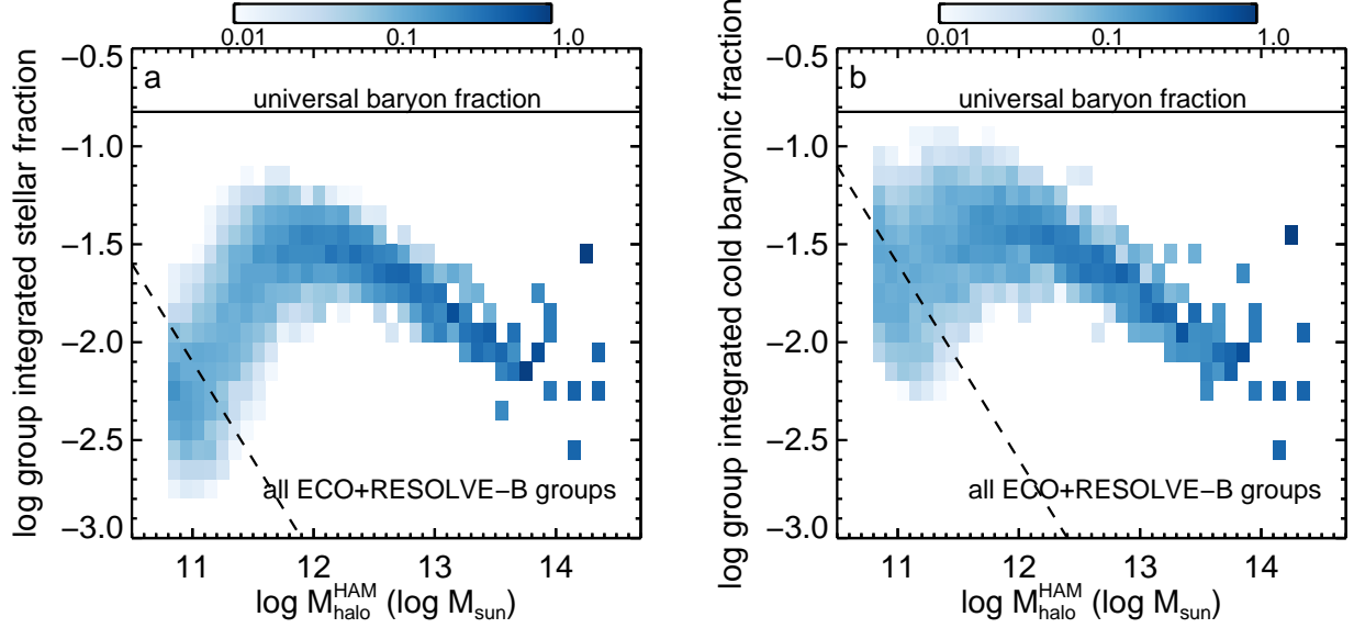
Figure 8. Same as Figure 7, except using M_{halo}^{HAM} based on group M_{star} abundance matching with scatter of 0.14 dex added (to match the scatter based on group luminosity). The group-integrated stellar fractions are similar to those using the group masses matched on L_r . The group-integrated cold baryon fractions have increased scatter at low masses compared to the L_r version. The increased scatter is likely due to the fact that L_r correlates more closely with cold baryonic mass than with stellar mass.
