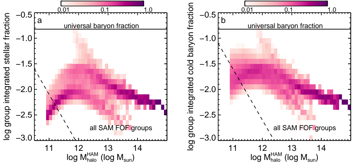
Figure 10. Conditional density plot of group-integrated (a) stellar and (b) cold baryon fraction for the SAM using the FOF groups with HAM based on group luminosity. We find that applying FOF and HAM to the SAM mock catalog results in the upside down U shape as seen in the ECO data. The spur of low cold baryon fraction groups for their halo mass is due to a population of galaxies with much lower masses than their luminosities would suggest. These are large, blue, star-forming galaxies, for which the dust correction does not sufficiently extinct their intrinsic magnitudes (see discussion in Gonzalez-Perez et al. submitted).
